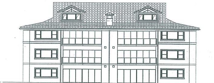
REAR ELEVATION
